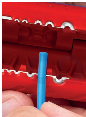
90 22 02 SB: Practical locator simplifies the insertion of single conductors for stripping
