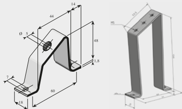
Montagewinkel Mounting Bracket
