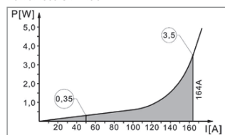
Power loss UVB 100
